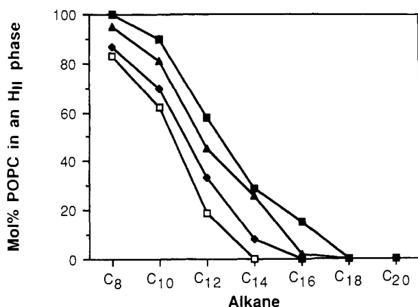
FIGURE 4: Phase equilibria in POPC- n -alkane- ^2\text{H}_2\text{O} systems as a function of the alkane chain length at four different temperatures: (□) 25, (◆) 35, (▲) 45, and (■) 55 °C. The water concentration was 49 wt % (54 mol/mol of POPC). The alkane concentration corresponds to 24 carbon atoms per lipid.
