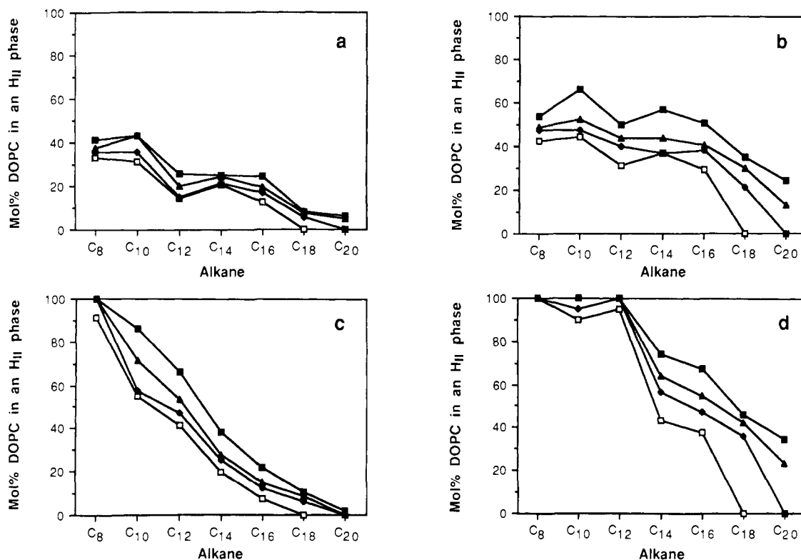
FIGURE 3: Phase equilibria in DOPC- n -alkane- ^2\text{H}_2\text{O} systems as a function of the alkane chain length at four different temperatures: (□) 25, (◆) 35, (▲) 45, and (■) 55 °C. The water concentration was 39 wt % (31 mol/mol of DOPC) in (a), 49 wt % (46 mol/mol of lipid) in (b), 35 wt % (31 mol/mol of DOPC) in (c), and 49 wt % (54 mol/mol of DOPC) in (d). The alkane concentration corresponds to 12 carbon atoms per lipid in (a) and (b) and 24 carbon atoms per lipid in (c) and (d). Eicosane ( \text{C}_{20} ) induced the formation of a phase giving rise to an isotropic ^{31}\text{P} NMR signal.
